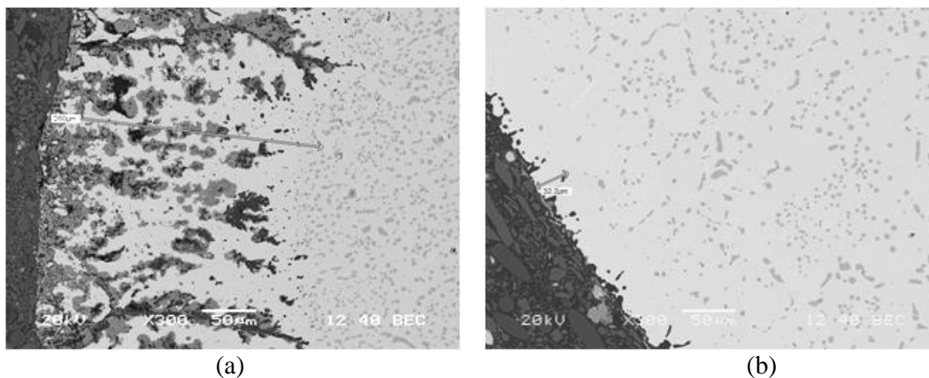
Figure 8. Low-depth subsurface oxidation of cross-rods from belts after 49 weeks in service, transverse cross-section: (a) belt B1 (standard atmosphere); (b) belt B2 (modified atmosphere).
