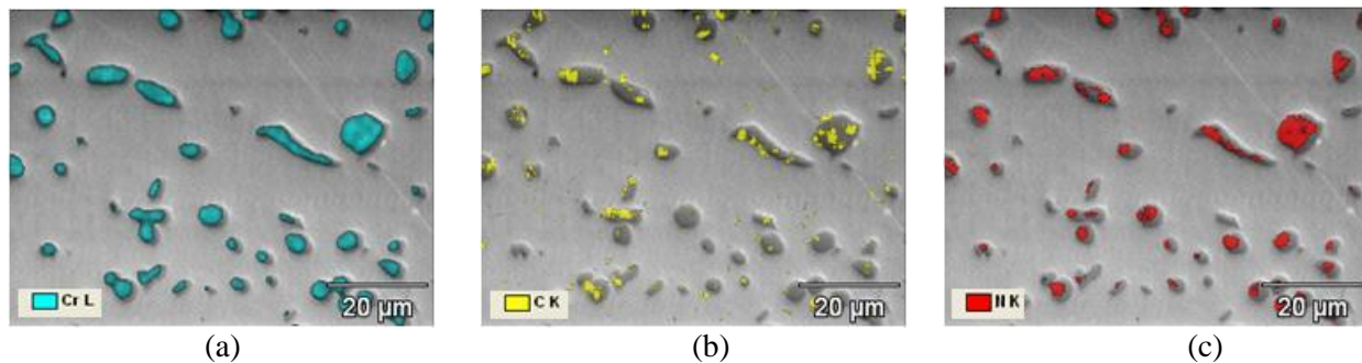
Figure 3. Transverse cross-section (central area) of the spiral wire from belt B1 after 49 weeks of service in the standard atmosphere, overlays of chromium (Cr), carbon (C) and nitrogen (N) on backscattered electron image, original magnification was 1500 times, accelerating voltage was 5 kV: (a) Cr (cyan); (b) C (yellow); (c) N (red).
