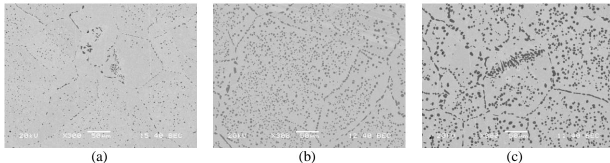
Figure 1. Representative microstructures of the central areas of the spiral wire B1 (standard atmosphere), transverse cross-sections, backscattered electron images (BEC): (a) 31 weeks in service; (b) 35 weeks in service; (c) 49 weeks in service.
