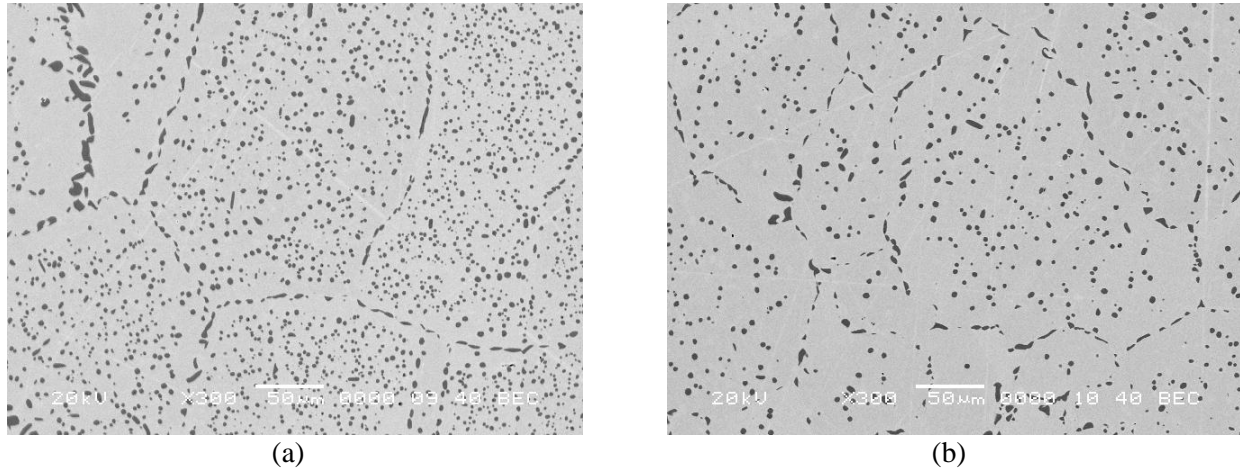
Figure 2. Central areas of the cross-rod after 35 weeks in service, transverse cross-sections, BEC: (a) belt B1 (standard atmosphere); (b) belt B2 (modified atmosphere).
