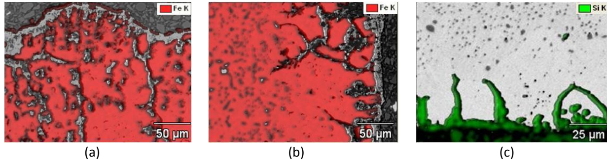
Figure 6. Surface and subsurface areas of spiral wires, transverse cross-sections, original magnification was 500 times, accelerating voltage was 20 kV, overlay of iron on BEC: (a) B1 after 49 weeks in service; (b) B2 after 49 weeks in service. Surface and subsurface area of a spiral wire from belt B2 after 35 weeks of service, original magnification was 1000 times, accelerating voltage was 5.0 kV, overlay of silicon on BEC (c).
