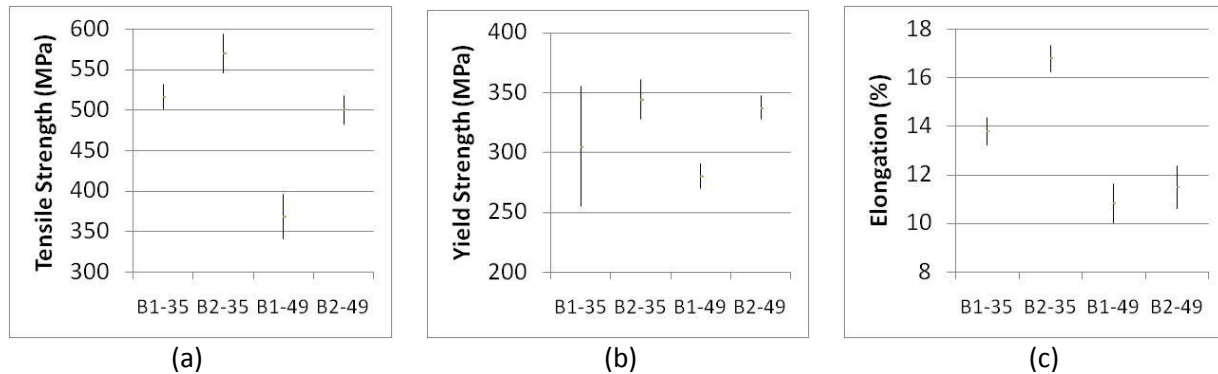
Figure 11. Tensile properties of cross-rods removed from belts B1 and B2; 95% confidence intervals for: (a) tensile strength; (b) yield strength; (c) elongation.
