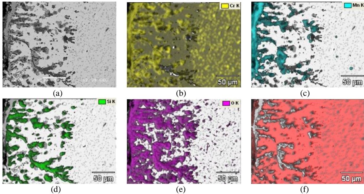
Figure 5. Surface and subsurface area of the spiral wire of belt B1 after 49 weeks in service, transverse cross-section, original magnification was 500 times, accelerating voltage was 20 kV: (a) backscattered electron image (BEC); (b) overlay of chromium on BEC; (c) overlay of manganese on BEC; (d) overlay of silicon on BEC; (e) overlay of oxygen on BEC; (f) overlay of iron on BEC.
