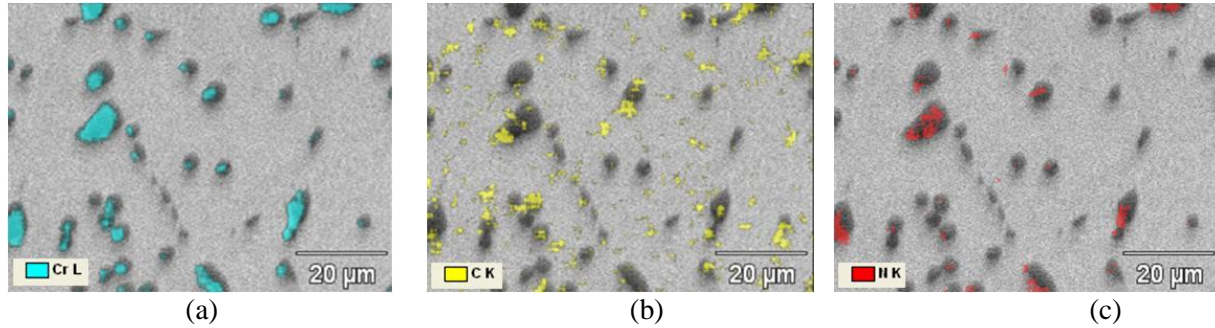
Figure 4. Transverse cross-section (central area) of the spiral wire from belt B2 after 49 weeks of service in the modified atmosphere, overlays of chromium (Cr), carbon (C) and nitrogen (N) on backscattered electron image, original magnification was 1500 times, accelerating voltage was 5 kV: (a) Cr (cyan); (b) C (yellow); (c) N (red).
